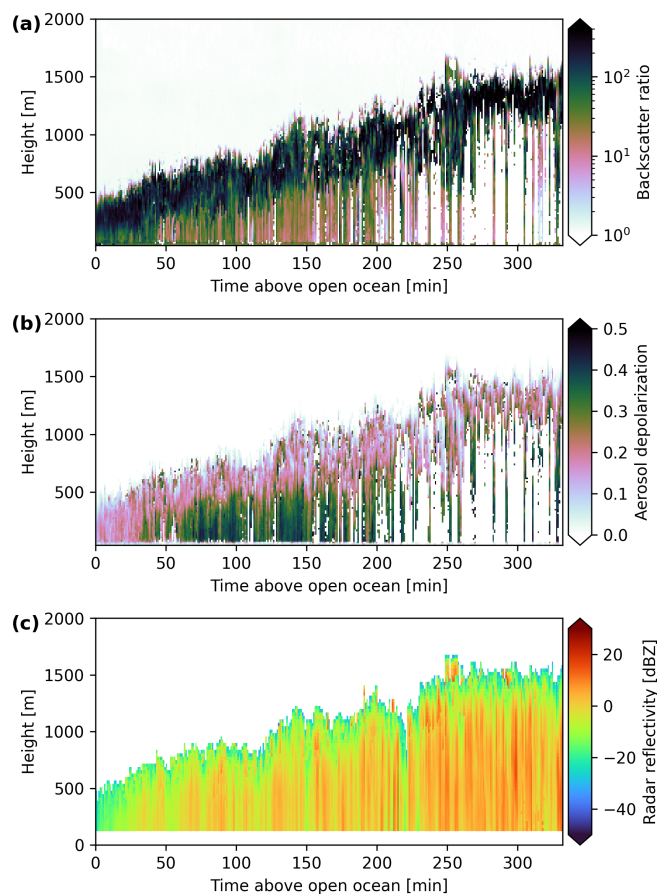
Figure 4. Lidar and radar measurements as a function of time above open ocean on 2022-04-01. (a) Lidar backscatter ratio. (b) Aerosol depolarization. (c) Radar reflectivity. The depolarisation data was filtered for cloud data only, with backscatter ratios larger than 10.
