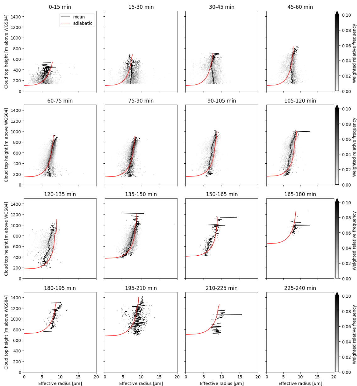
Figure 5. Vertical profiles of the effective radius of liquid cloud droplets for different time ranges above open ocean. The black solid line indicates the mean measured effective radius. The red solid lines are vertical profiles calculated using the parcel model (Sect. 2.2).
