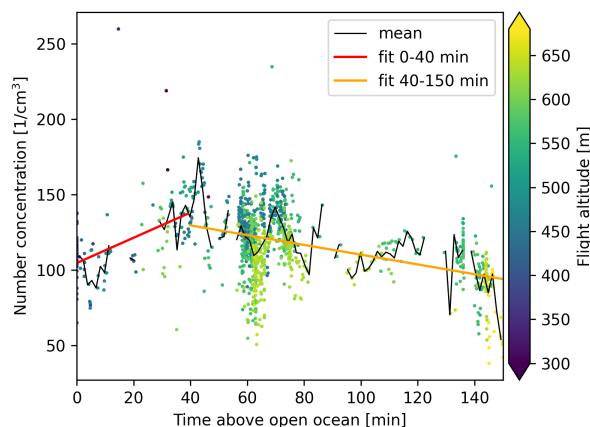
Figure 6. Cloud droplet number concentration as a function of time above open ocean from in situ measurements. The color coding denotes the height of the measurements. The red and orange solid lines are linear fits to the data for times smaller and larger than 40 min, respectively. Only measurements with a LWC larger than 0.1 \text{ gm}^3 and with a sea ice concentration smaller than 80 % were used.
