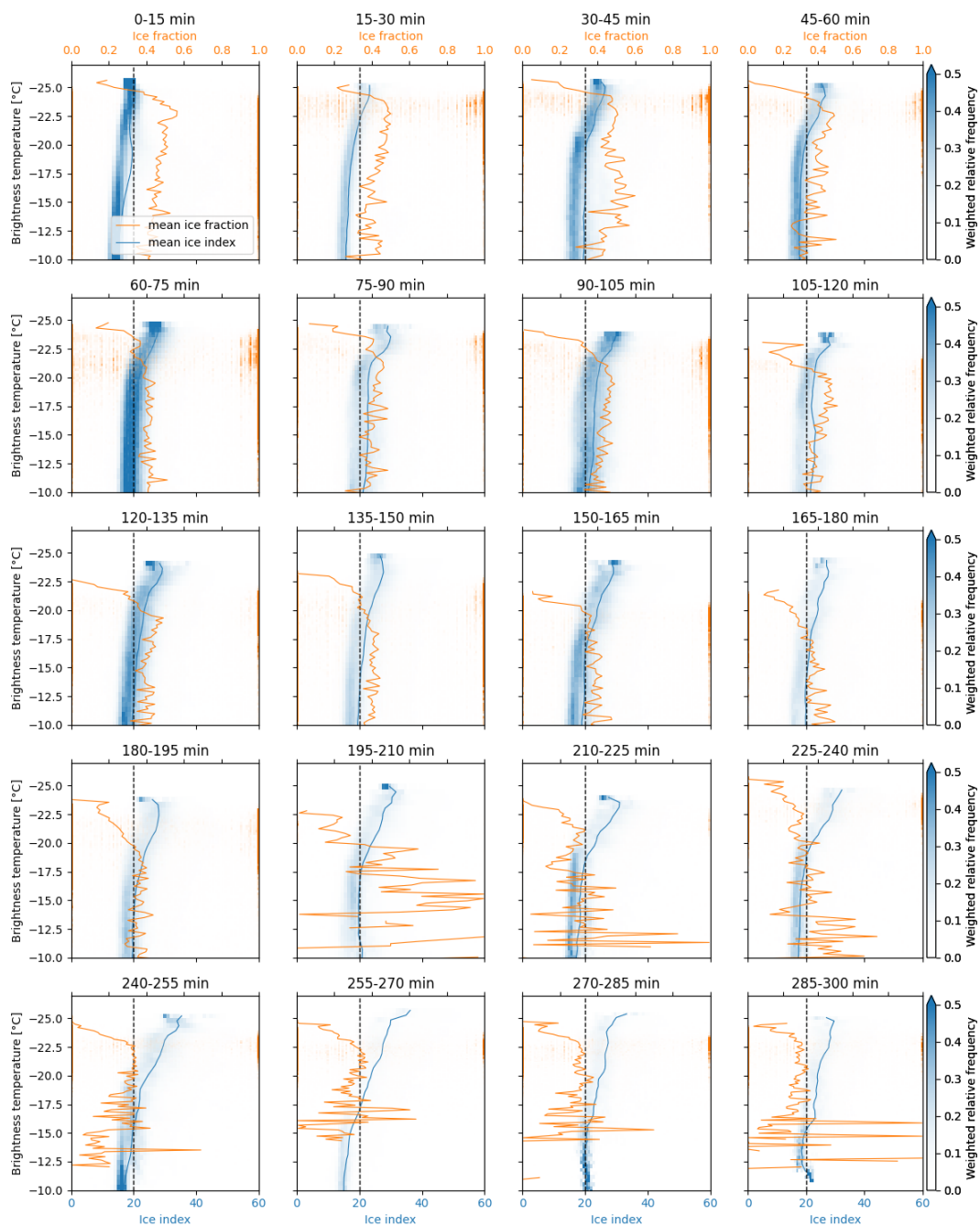
Figure 2. Histograms of ice index (blue) and ice fraction (orange) as a function of the brightness temperature between 7.7 \mu\text{m} and 12 \mu\text{m} (representative for cloud top) for different time ranges above open ocean. The blue and orange solid lines denote the respective mean. The black dashed line indicates the threshold value of the ice index between the liquid water and the mixed phase. The ice fraction was derived with the IDEFAX for the slope angular range.
